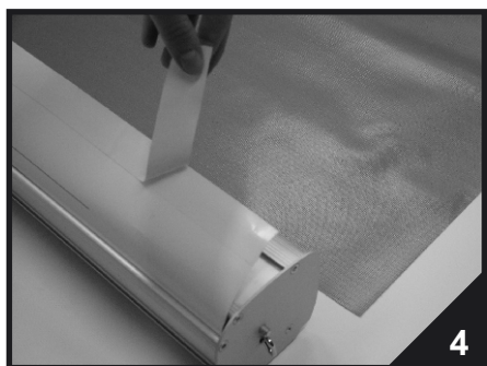
4. Remove the covering tape from the base unit.
